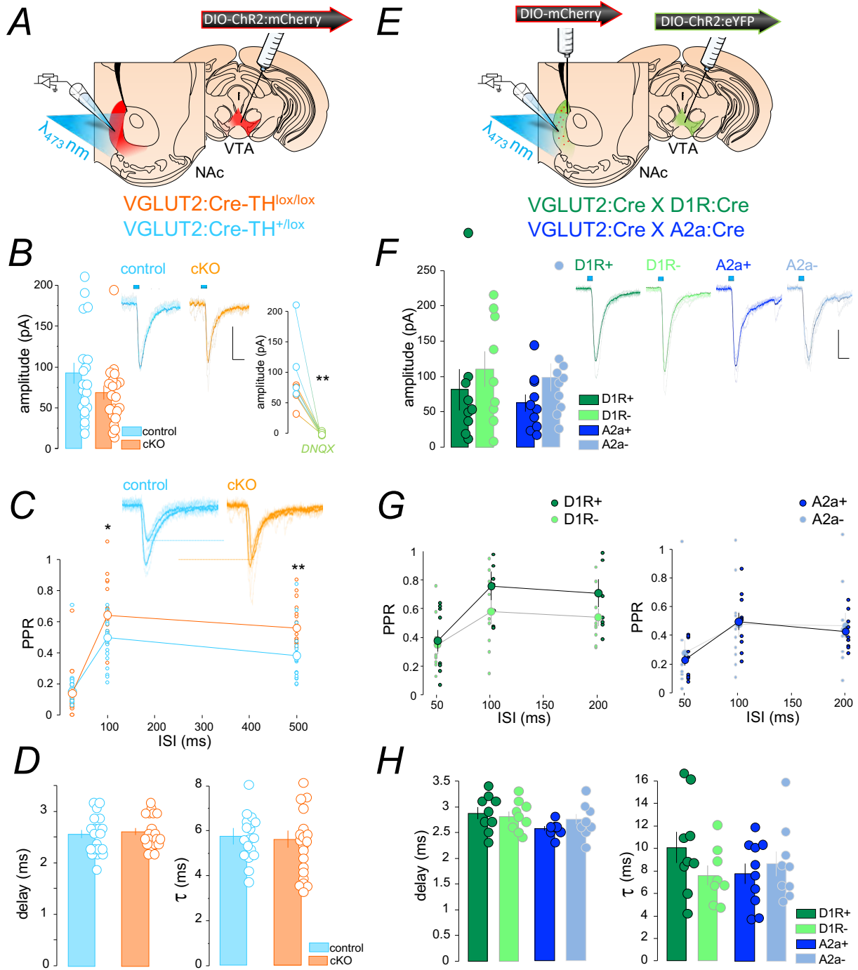
Figure S3 (relates to Figure 1). Glutamate transmission is intact in cKO mice and VTA glutamate neurons similarly target D1- and D2-expressing NAc MSNs. A. Schematic for ex vivo electrophysiology measure of photo-evoked glutamate currents. B. Single pulse photostimulation (5 ms) of VTA terminals-triggered oEPSCs in NAc neurons of similar amplitude in control (n=20 cells) and cKO mice (n=21; t-test, p=0.12); blocked by 10 \mu M DNQX; t-test, **p=0.002 (n=8 cells). Insets show example traces recorded in control and cKO mice; scale 50
