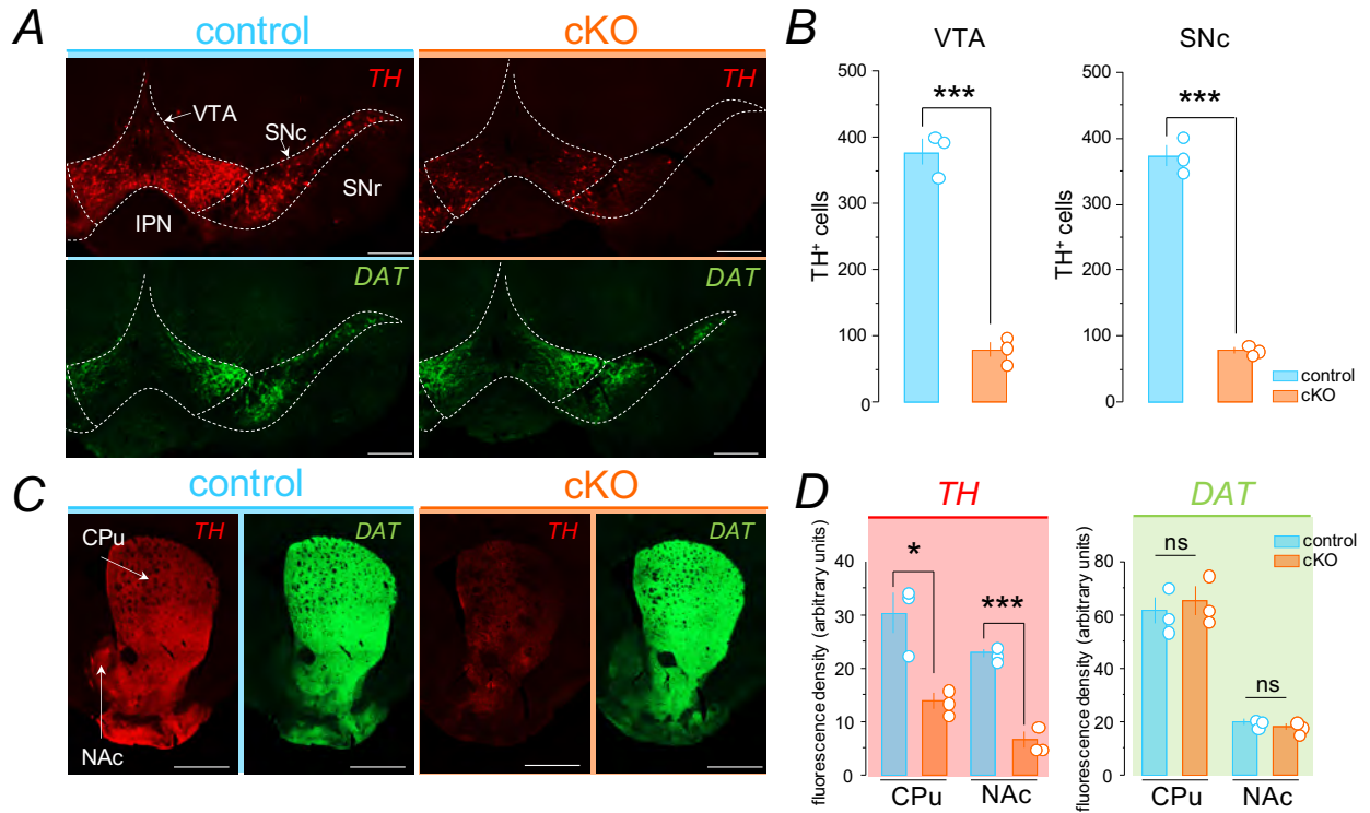
Figure S1 (relates to Figure 1). Reduced TH expression in cKO. A. Coronal midbrain sections containing VTA and substantia nigra pars compacta (SNc) DA neurons in control (left) and cKO (right) mice demonstrate fewer TH-expressing neurons but comparable DAT expression appears unchanged; scale: 500 \mu m. B. Cell counts reveal ~80% reduction in the number of TH immunolabeled cells in the VTA and SNc of cKO compared to controls; t-test, *** p < 0.001 ( n = 3 mice). C. Coronal sections through striatum show TH and DAT expression in DA terminals of caudate/putamen (CPu) and nucleus accumbens (NAc) of control (left) and cKO mice (right); scale: 500 \mu m. D. Densitometric analysis of immunofluorescent signal shows reduced TH but unchanged DAT expression in cKO mice; t-test, * p = 0.015 , *** p = 0.0006 ( n = 3 mice/group). Data are represented as mean \pm SEM.
