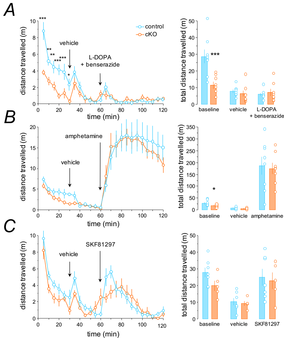
Figure S2 (relates to Figure 1). Responses to DA agonists in control and cKO mice. A.
