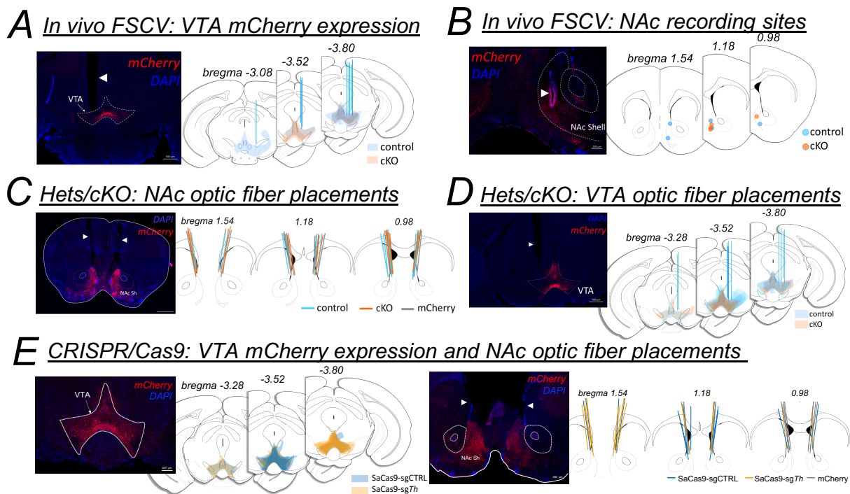
Figure S4 (relates to Figures 1-4). Post hoc histological assessment of expression and implant sites. A. Coronal section of ChR2:mCherry expression in VGLUT2-Cre neurons in VTA with optic fiber tract (arrowhead); schematic of optic fiber placements (related to Figure 1I ). B. Coronal section showing ChR2:mCherry expression in medial NAc shell with lesion made following FSCV recordings (arrowhead); FSCV recording sites (related to Figure 1I ). C. Coronal section showing bilateral optic fiber tract (arrowheads) and ChR2:mCherry expressing VTA glutamate terminals in medial NAc shell of control and cKO mice; fiber optic placements (related to Figure 2A-C and 3A-C ). D. Coronal section showing expression of ChR2:mCherry in glutamate neurons in VTA and optic fiber placement (arrowhead); schematic illustrating optic fiber placements and expression of ChR2:mCherry (related to Figure 2D-F and 3D-F ). E. Left: Coronal section of ChR2:mCherry expression in VGLUT2-Cre neurons in VTA. Right: fiber optic placements in medial NAc shell (related to Figure 4F-H ).
